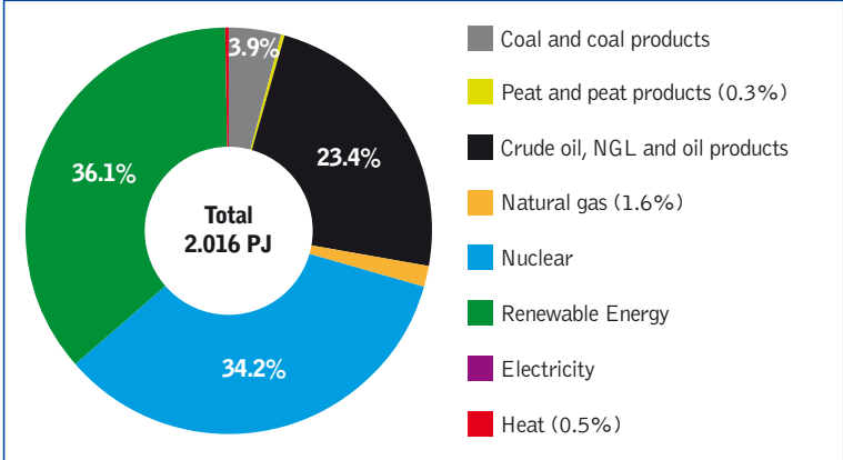
Figure 47: Total primary energy supply in Sweden in 2014 (Source: World Energy Balances © OECD/IEA 2015)
