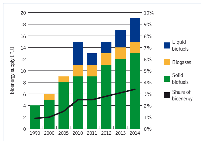
Figure 37: Development of total primary energy supply from bioenergy in Ireland 1990 – 2014 (Source: Renewables Information © OECD/IEA 2015)
