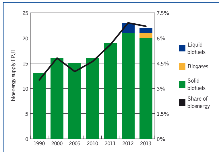
Figure 16: Development of total primary energy supply from bioenergy in Croatia 1990 – 2013 (Source: Renewables Information © OECD/IEA 2015)
