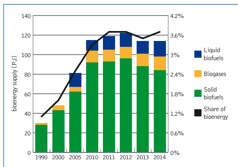
Figure 46: Development of total primary energy supply from bioenergy in the Netherlands 1990 – 2014
