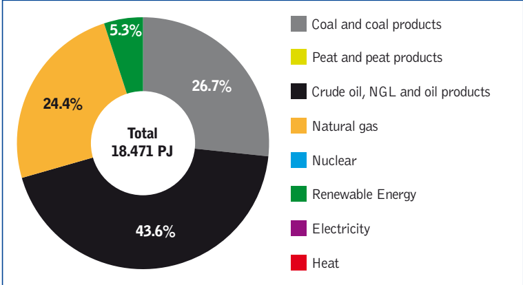
Figure 71: Total primary energy supply in Japan in 2014 (Source: World Energy Balances © OECD/IEA 2015)
