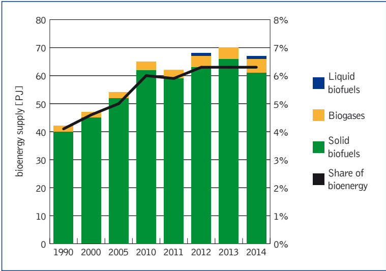
Figure 94: Primary bioenergy supply in Switzerland 1990 – 2014 (Source: Renewables Information © OECD/IEA 2015)
