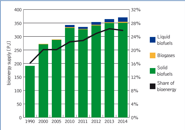
Figure 24: Development of total primary energy supply from bioenergy in Finland 1990 – 2014 (Source: Renewables Information © OECD/IEA 2015)
