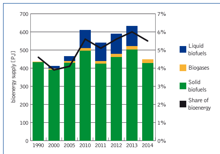
Figure 29: Development of total primary energy supply from bioenergy in France 1990 – 2014 (Source: Renewables Information © OECD/IEA 2015)
