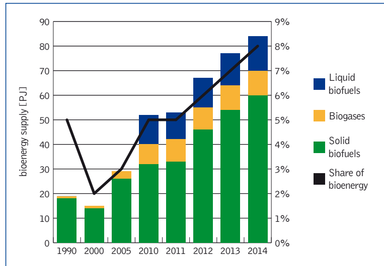
Figure 78: Development of total primary energy supply from bioenergy in Korea 1990 – 2014 (Source: Renewables Information © OECD/IEA 2015)
