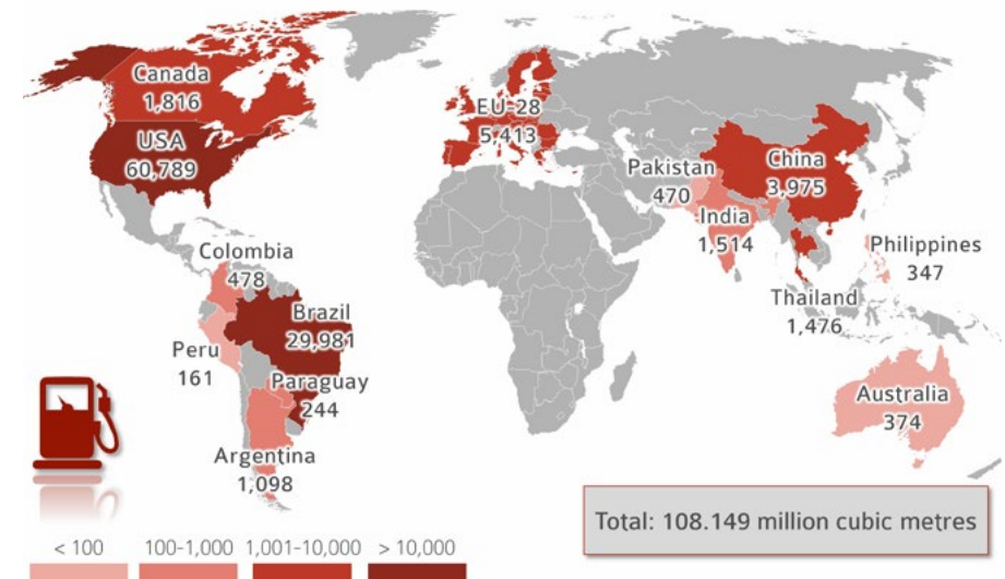
Bioethanol production in key countries, in 2018, in 1,000 cubic metres
