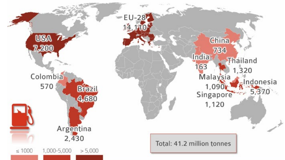
Biodiesel production in key countries, in 2018, in 1,000 tonnes
