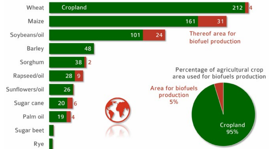
Shares of total cultivation area (arable land + permanent crops) used for selected crops for biofuel production, worldwide, in 2018, in million hectares © AMI 2019 Source: OECD, USDA, Oil World
